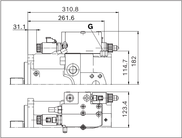
▼ DRL – Pressure controller, parallel operation
