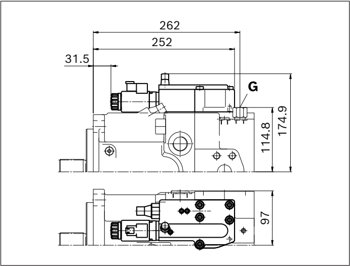
▼ DRS/DRG – Remote-controlled pressure controller, load sensing
